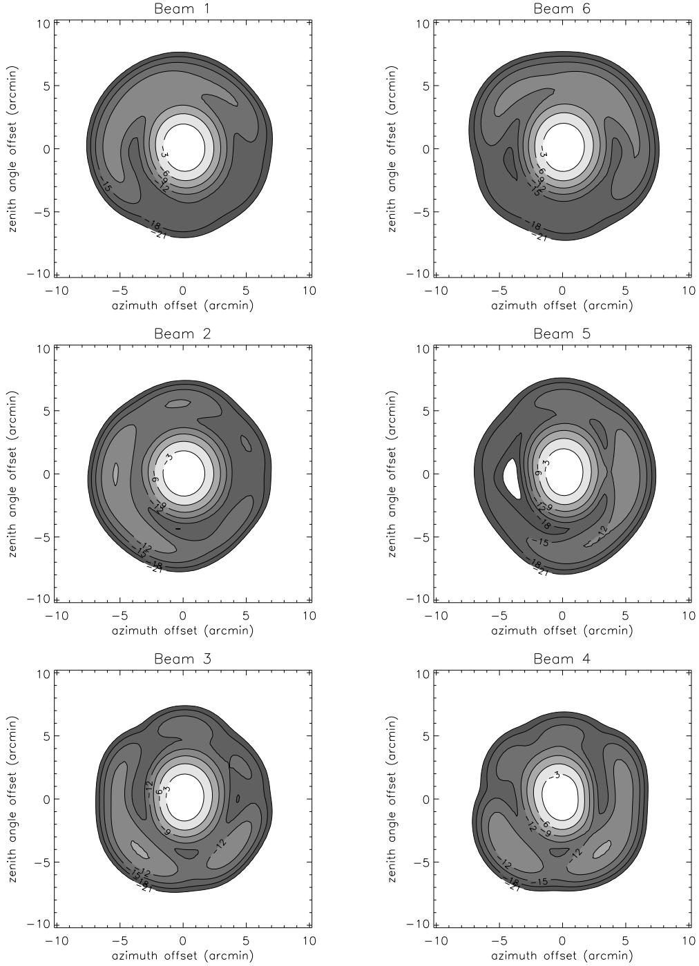
Fig. 4.— Beam patterns of the six peripheral ALFA beams. Contour lines and shading intervals are plotted at intervals of 3 dB below peak response (the highest contour is at half the peak power). Note that the sidelobe levels are significantly larger than for the central beam 0, and that they rise steeply on the outer side of the array, exhibiting strong comatic aberration.
