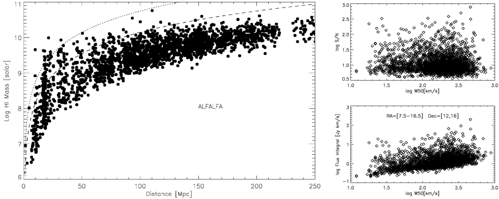
Fig. 2. – Left: Spänhauer plot HI sources in the region R.A.=[ 7.5^h – 16.5^h ], Dec=[ 12^\circ – 16^\circ ]. The two smooth lines identify the completeness limit (dotted) and the detection limit (dashed) for sources of 200 \text{ km s}^{-1} linewidth for the HIPASS survey. Note that due to rfi, ALFALFA is effectively blind in the redshift range between approximately 15000 and 16000 \text{ km s}^{-1} . Right: Signal-to-noise ratio vs. velocity width (top) and Flux integral vs. velocity width for the galaxies in the left-hand panel.
