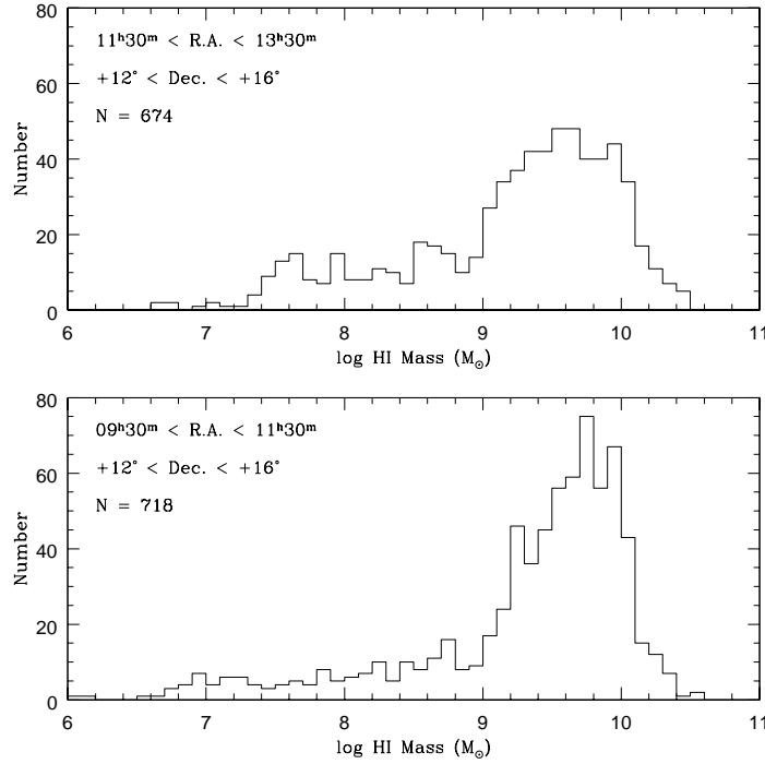
Figure 2. Left: Upper: Histogram of the HI masses for ALFALFA sources in the region 11^h 30^m < \text{R.A.} < 13^h 30^m , +12^\circ < \text{Dec.} < +16^\circ including the Virgo cluster region. All objects with cz < 3000 \text{ km s}^{-1} and found within 5^\circ of M87 are placed at the Virgo distance of 16.7 Mpc.. Lower: Similar histogram over the same declination band but in the range 09^h 30^m < \text{R.A.} < 11^h 30^m .
