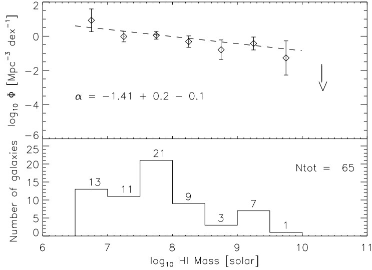
Figure 6: The HIMF for the Leo I group with a linear fit overplotted. The number of low HI mass objects in the Leo I sample is much larger than that used in previous determinations of the HIMF (more than twice as many as in the entire HIPASS sample); there are no massive HI galaxies in Leo. The low mass slope is steeper than that determined for the optical luminosity function. From Stierwalt et al. (2009).
