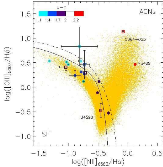
Figure 5: Location of the HI rich early type galaxies in the typical optical line diagnostic diagram used to distinguish star forming and active galaxies. From Grossi et al. (2009).
